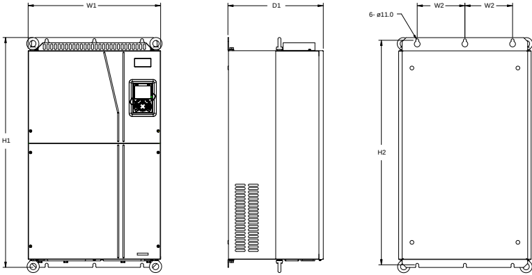
图 C-7 132G/160P~200G/220P 壁挂安装
