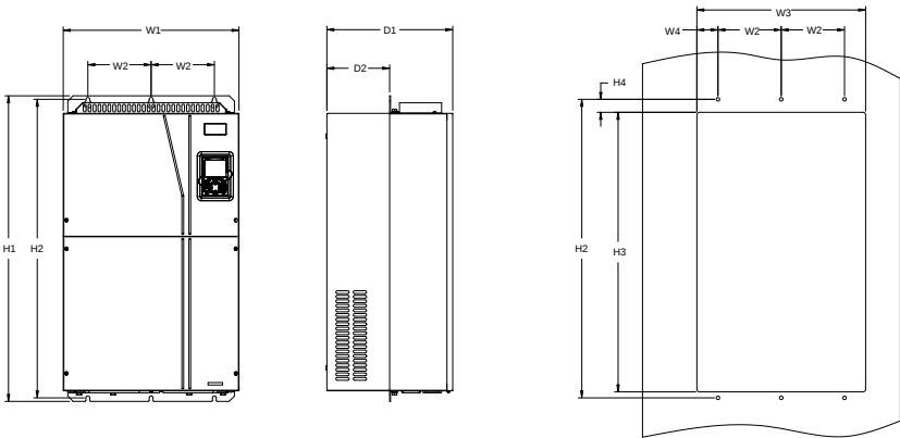
图 C-11 132G/160P~200G/220P 法兰安装
